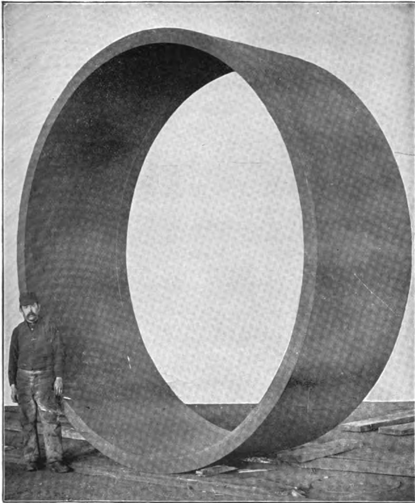
FIG. 2. —Specimen Steel Ring, Hydraulically Forged without Weld. (Outside dia., 11 ft. 7 \frac{3}{8} in.; width, 4 ft. 3 \frac{1}{4} in.; thickness, 5 \frac{1}{4} in.)
