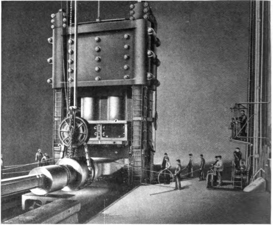
ARMOR-PLATE PRESS (PRESSURE 14,000 TONS TO SQUARE INCH). USED IN FORGING PLATES FOR HARVEYZED STEEL VAULT CONSTRUCTION
