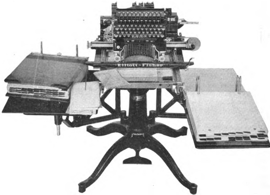
LEDGER POSTED, DEPOSITORS' STATEMENT AND JOURNAL OF CHECKS AND DEPOSITS ALL MADE AT ONE OPERATION
